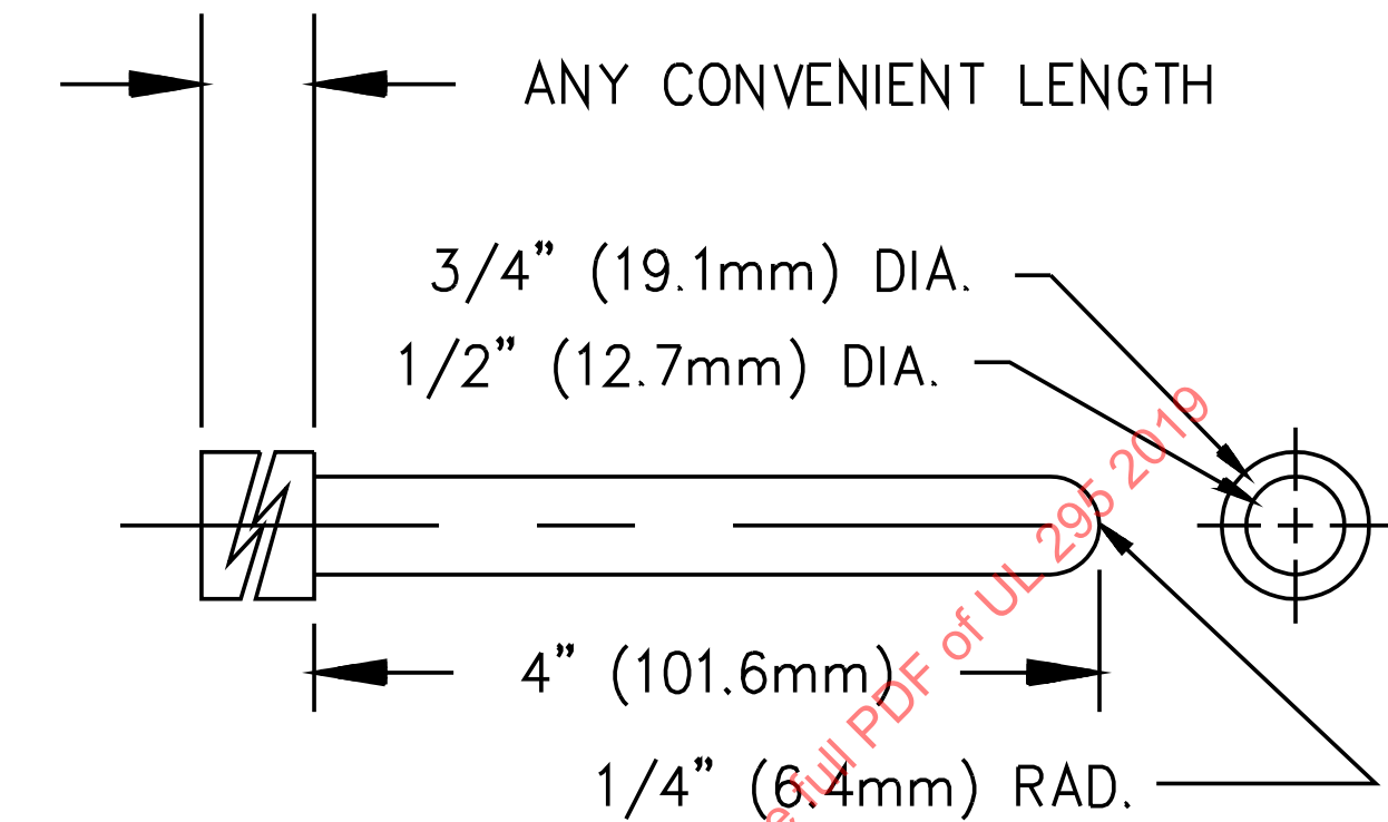
Figure 9.2 Probe for film-coated wire
