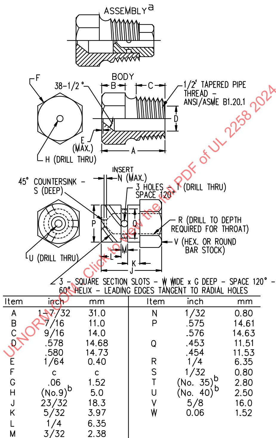
Figure 9.2.7.1 RAIN TEST SPRAY HEAD
