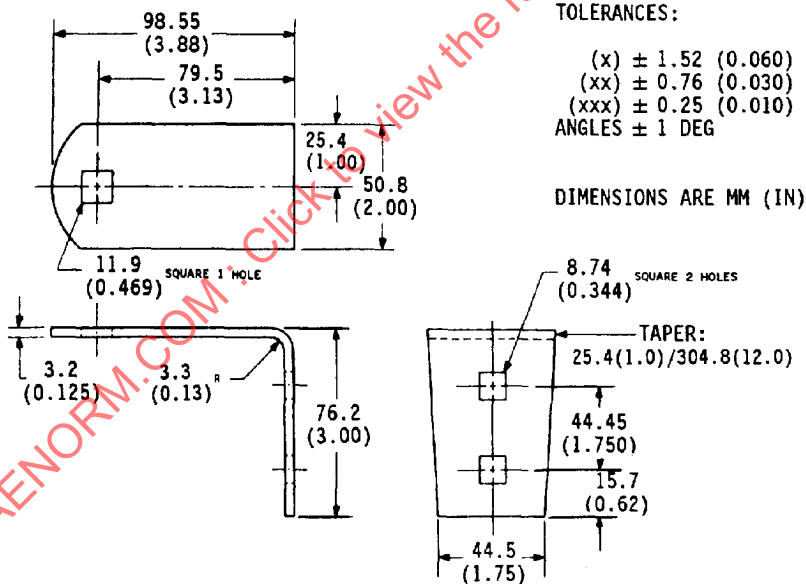
FIGURE 3—BRACKET FOR WARNING LAMP
