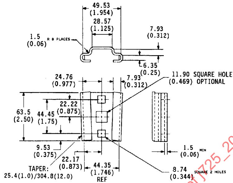
FIGURE 2—SOCKET
