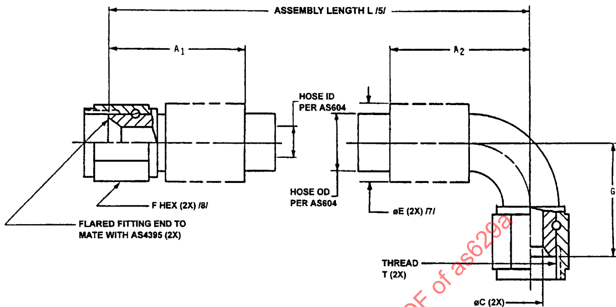
FIGURE 1 - HOSE AND FITTING DIMENSIONS
