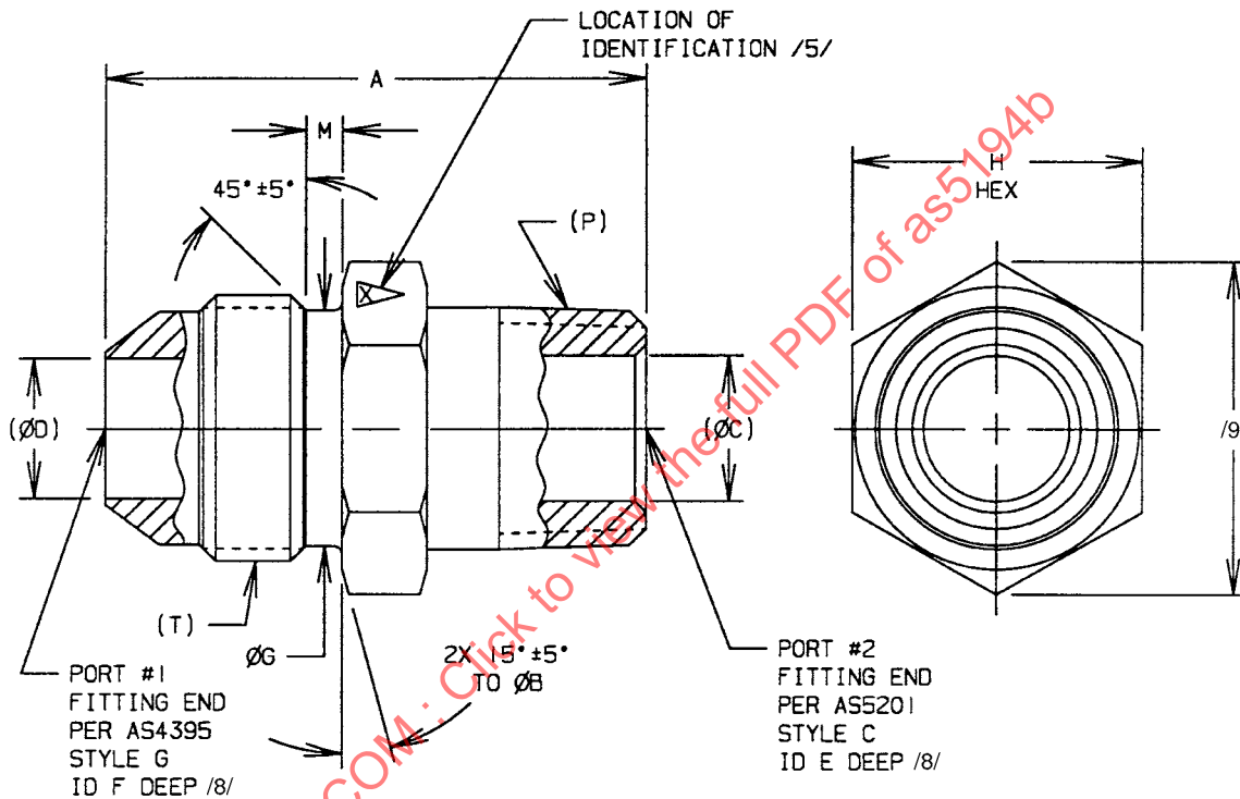
FIGURE 1 - FITTING, ADAPTER
