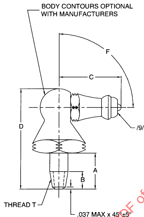
FIGURE 3 - FITTING, ELBOW, 90°
