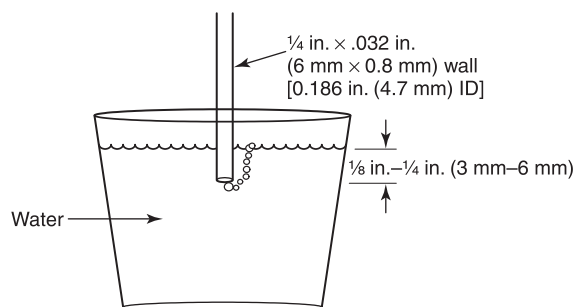
▲ FIGURE A.7.5.14(c) Leak Test for a Safety Shutoff Valve. [86:Figure A.7.4.9(c)]
