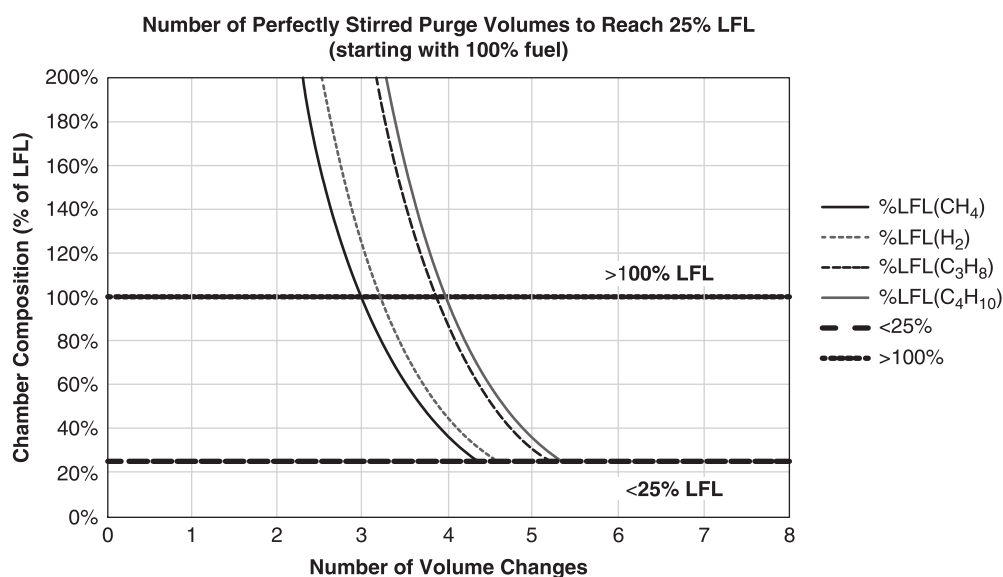
N FIGURE A.8.5.1.1(1) Composition Profile for Four Fuel Gases Undergoing Fresh-Air Purging.
