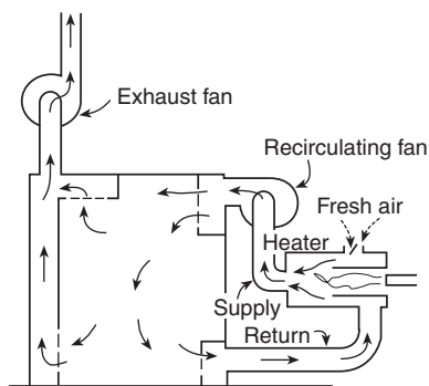
FIGURE A.3.3.33.3(b) Example of a Direct-Fired, External, Recirculating-Through Heater.
