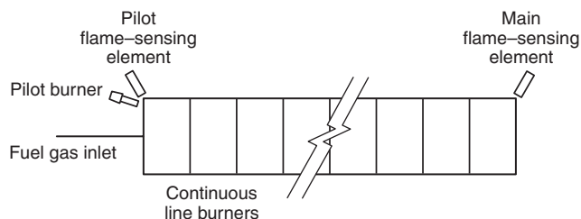
FIGURE A.8.10.6(a) Example of a Combustion Safeguard Supervising a Pilot for a Continuous Line Burner During Light-Off and the Main Flame Alone During Firing.
