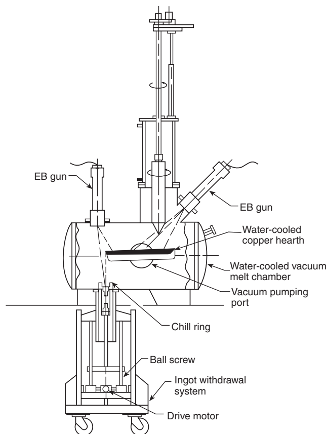
FIGURE A.1.1.6(e) Example of an Electron-Beam (EB) Melter.
