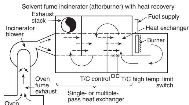
FIGURE A.10.6.2 Example of a Direct Thermal Oxidation Incinerator (Afterburner) with Primary Heat Recovery.
