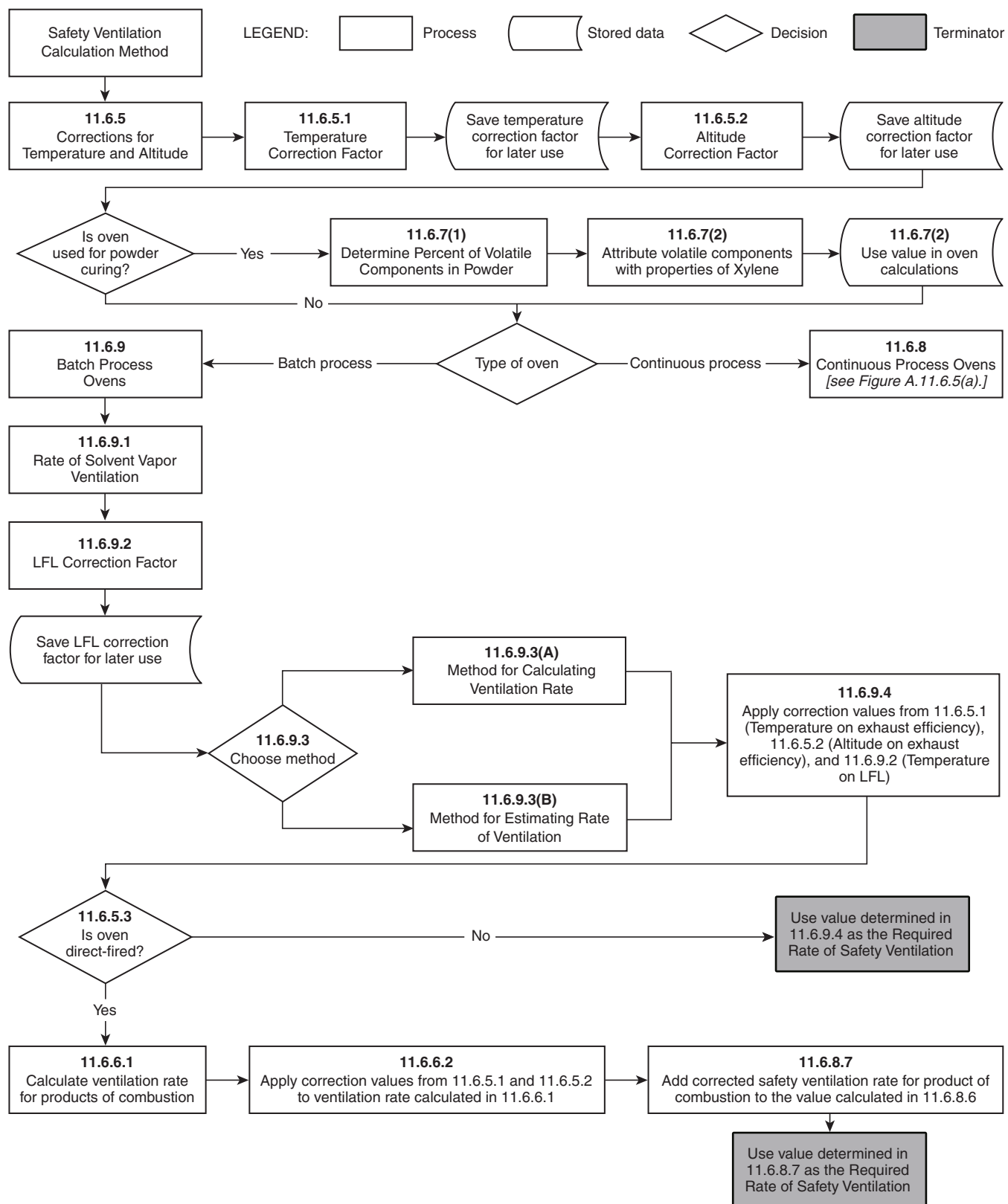
FIGURE A.11.6.5(b) Calculation of Required Safety Ventilation for Batch Process Ovens.
