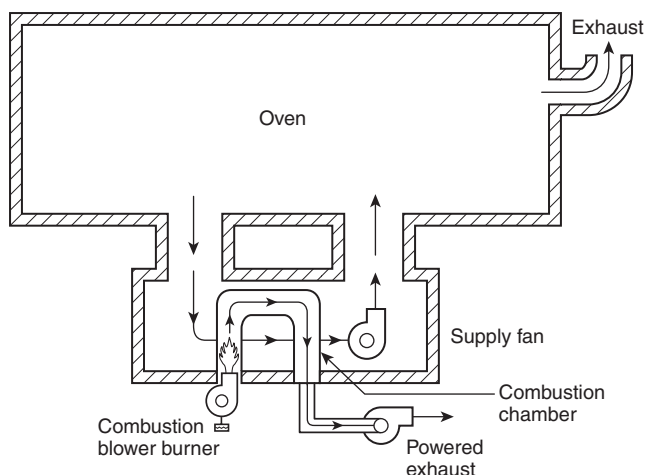
FIGURE A.5.3.1(6) Example of a Non-Recirculating, Indirect-Fired Oven.
