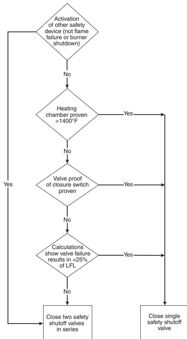
FIGURE A.8.8.1.3 Safety Shutoff Decision Tree.
