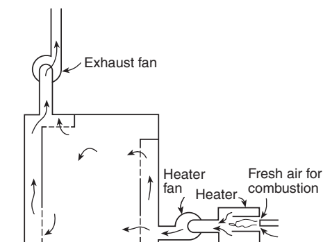
FIGURE A.3.3.33.3(a) Example of a Direct-Fired, External, Nonrecirculating Heater.
