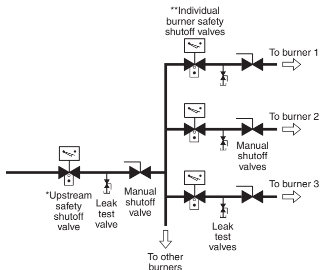
FIGURE A.8.8.1.2 Multiple Burner System Using Proof-of-Closure Switches.
