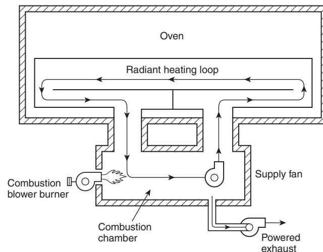
FIGURE A.3.3.33.6 Example of an Indirect-Fired Internal Heating System.
