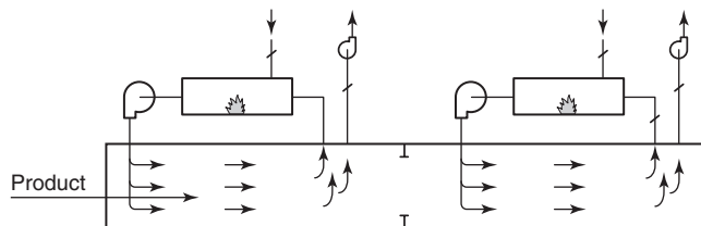
FIGURE A.11.6.10.3(a) Two Heating Zones — Separate Exhaust Fans.
