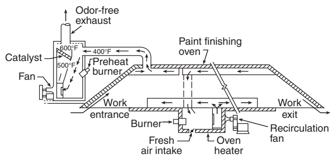
FIGURE A.10.6.4(a) Example of Catalyst System Independent of Oven Heater for Air Pollution Control.
