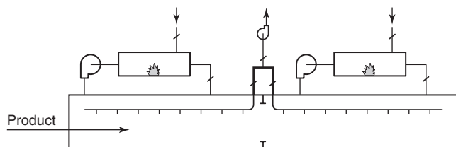
FIGURE A.11.6.10.3(c) Two Heating Zones — Common Exhaust Fan.
