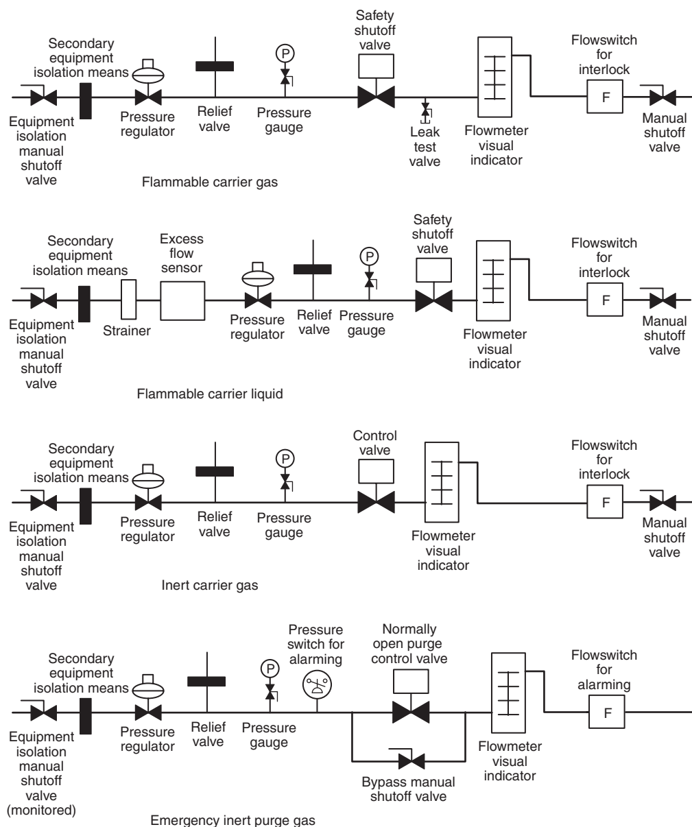
FIGURE A.13.5.11.10 Examples of Special Atmosphere Equipment Piping.
