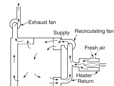
FIGURE A.3.3.33.3(c) Example of a Direct-Fired, External, Recirculating-Not-Through Heater.
