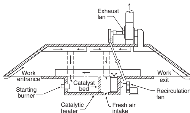
FIGURE A.10.6.4(b) Example of Indirect-Type Catalytic Oven Heater for Full Air Pollution Control.
