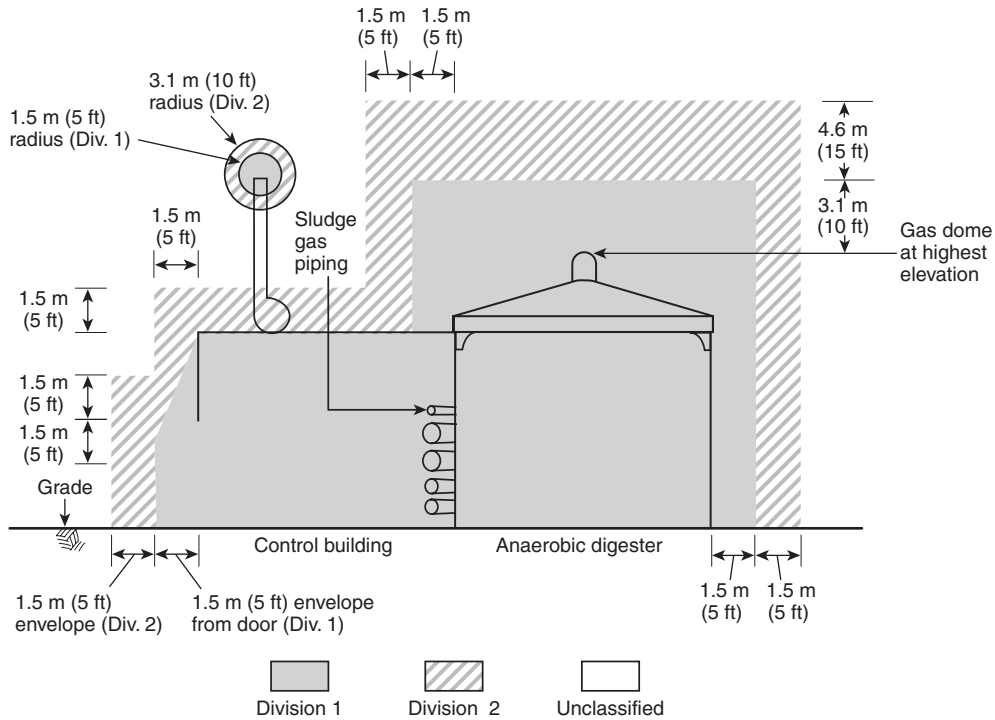
FIGURE A.6.2(b) Anaerobic Digester Control Building Containing Sludge Gas Piping and Using Ventilation Method (A); Illustration of Table 6.2(a), Row 16a.
