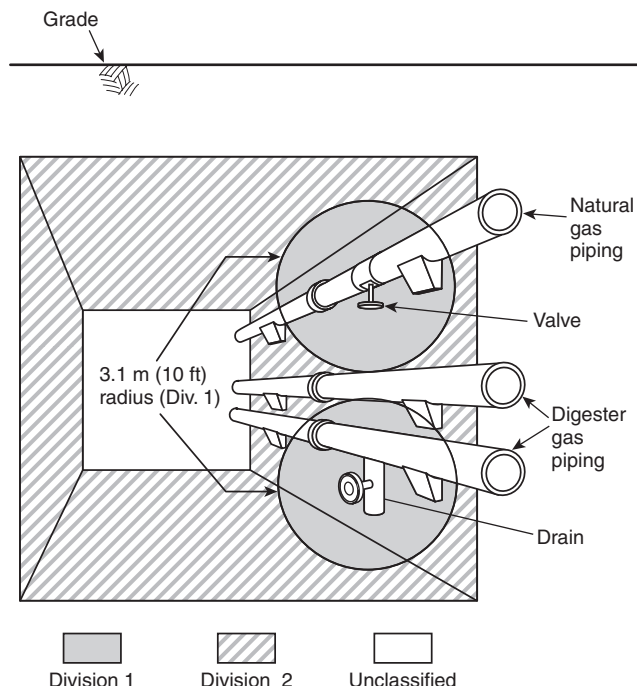
FIGURE A.6.2(f) Underground Tunnel Containing Natural Gas or Sludge Gas Piping and Using Ventilation Method (D); Illustration of Table 6.2(a), Rows 20a and 20b.
