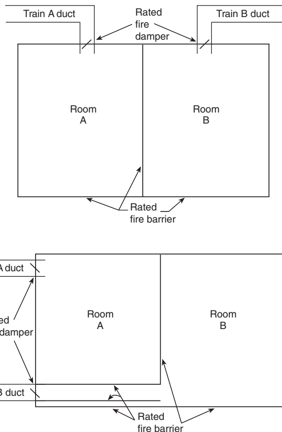
FIGURE A.8.4.8.2 Typical Air Duct Fire Damper Configuration.
