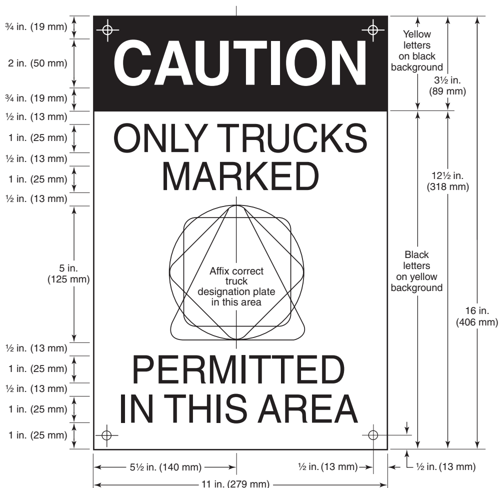
FIGURE 9.4.2.1 Building Sign for Posting at Entrance to Hazardous Areas.
