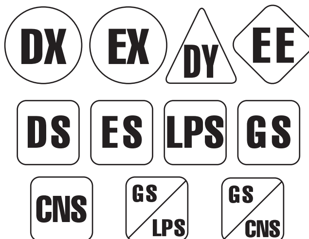
FIGURE 9.4.1.2.1 Markers Used to Identify Types of Industrial Trucks.
