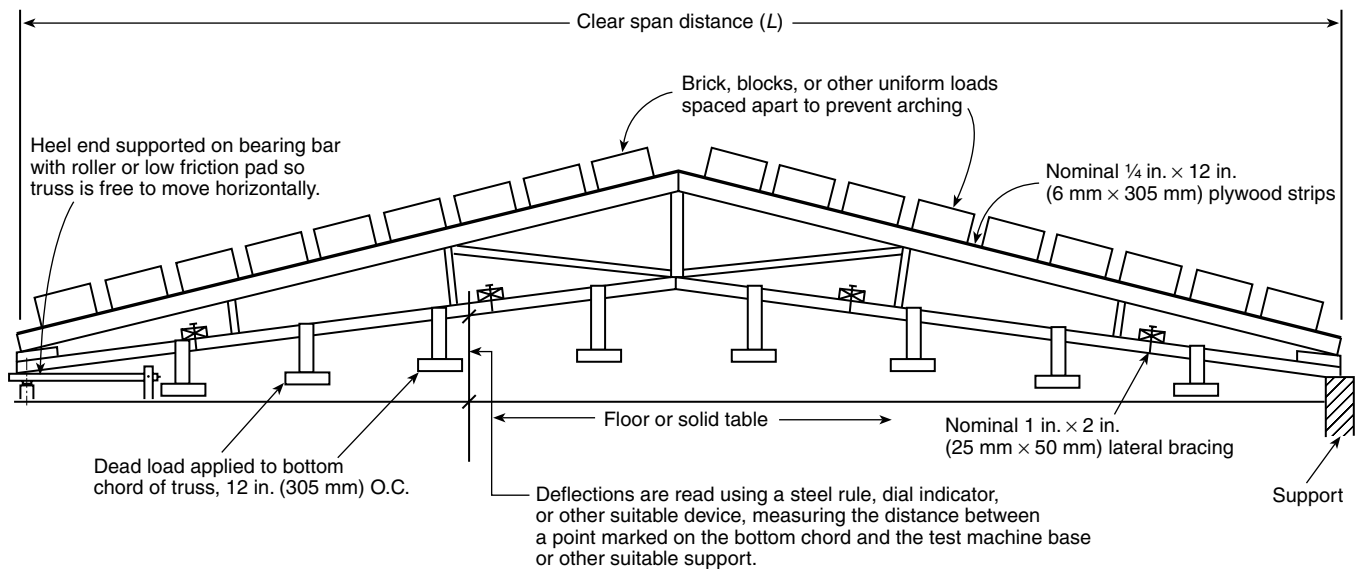
FIGURE 5.2.2.2 Test setup for roof trusses tested in groups of two or more.
