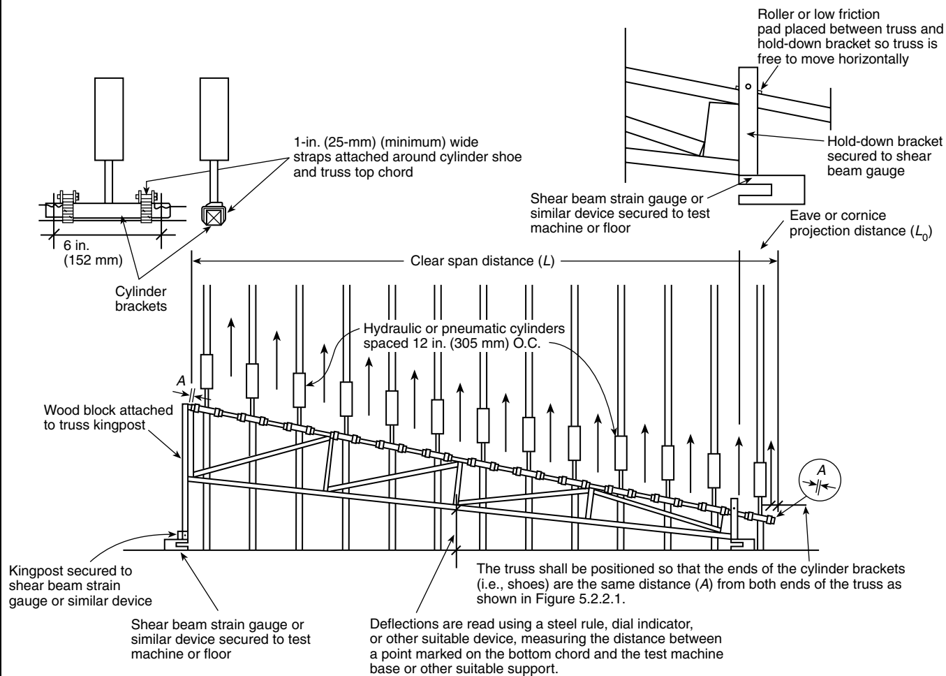
FIGURE 5.2.5.1 Uplift load test fixture.
