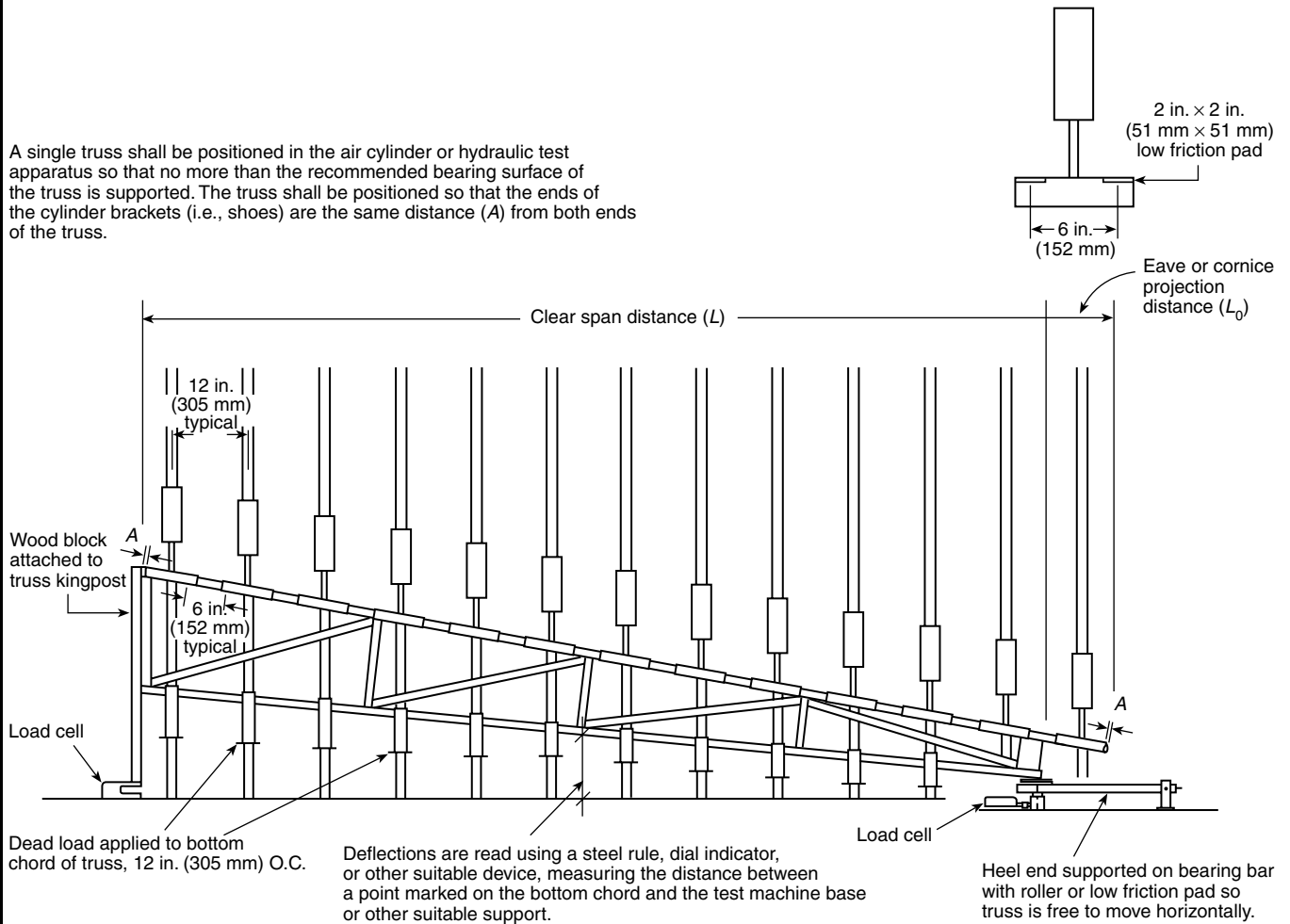
FIGURE 5.2.2.1 Test fixture for testing trusses singly.
