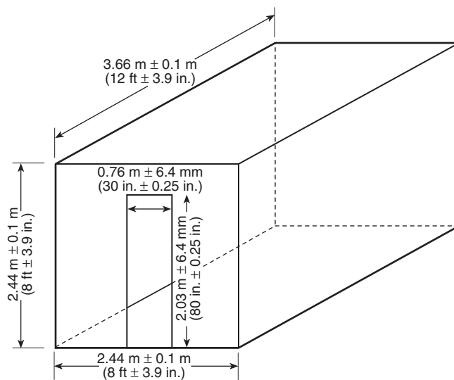
FIGURE 4.2 Interior Room Dimensions and Interior Doorway Dimensions.
