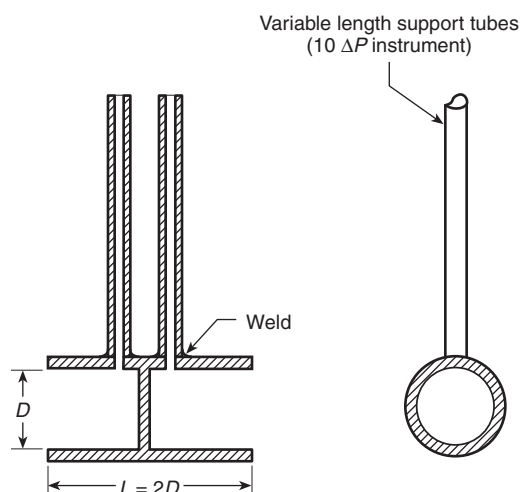
▲ FIGURE 7.3.2.1 Bidirectional Probe.
