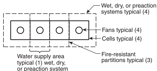
FIGURE A.5.6.2.1 Multiple Wet, Dry, or Praction Systems with Fire-Resistant Partitions.
