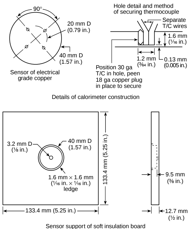
FIGURE 6-10.4.1.10 Sensor assembly.
