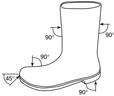
FIGURE 6-5.5.2 Test areas.
