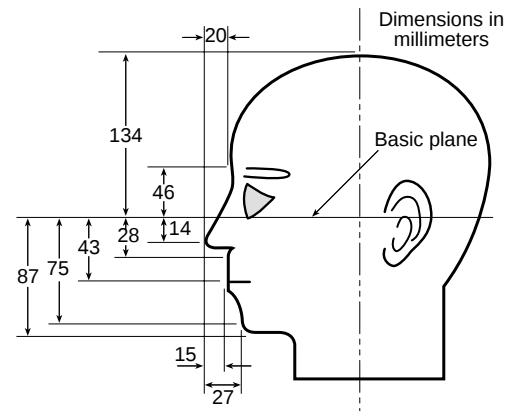
FIGURE 6-17.4.1.1 Alderson headform.
