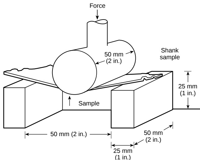
FIGURE 6-40.4.4 Shank bend test setup.
