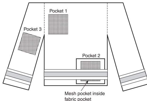
N FIGURE 12.9.1.4 Design and Locations of Sample Mesh Pockets on Surrogate Coats.
