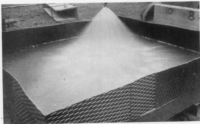
Representative types of spray nozzles installed above tanks to protect open surfaces of flammable liquids.
