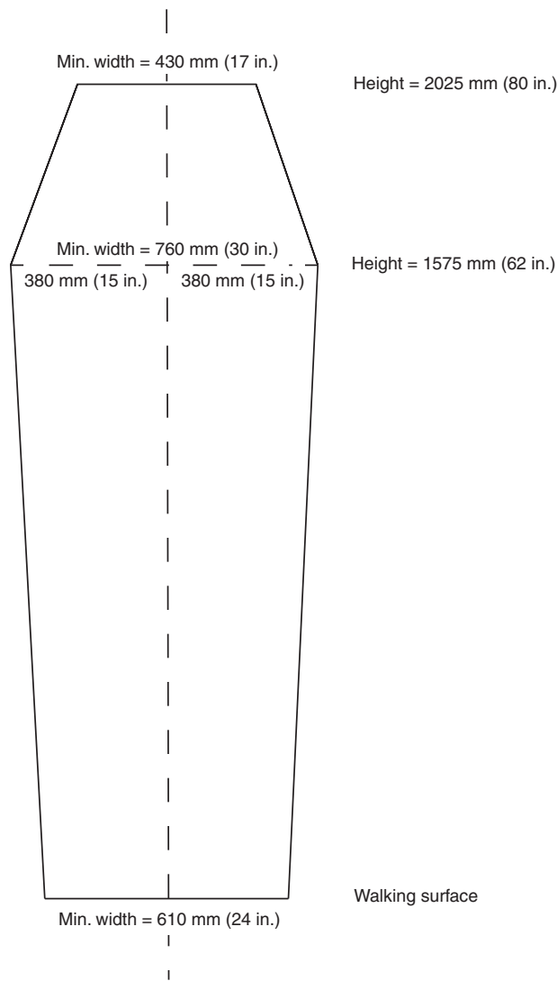
Δ FIGURE A.6.3.2.1 Unobstructed Clear Width for Trainway Walkway.
