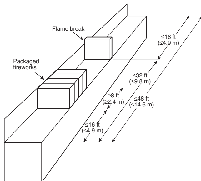
FIGURE A.7.3.15.3.3 Packaged Fireworks Merchandise and Flame Break Requirements.
