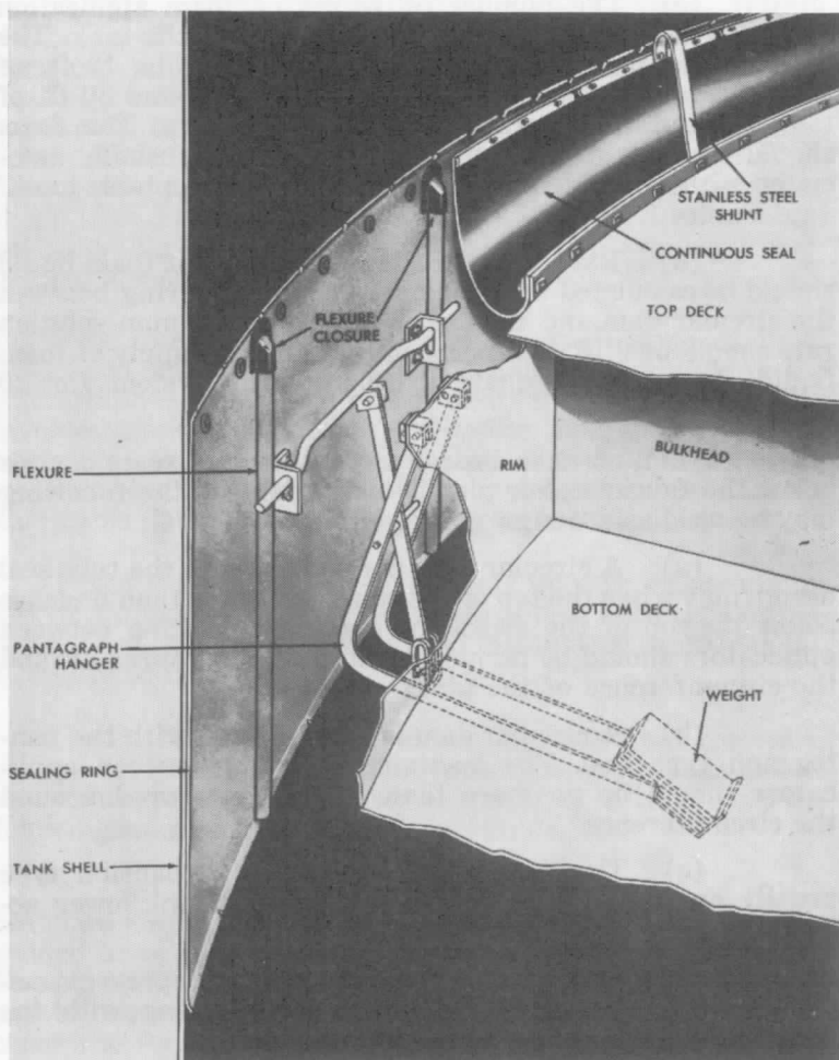
Fig. A-3311(1). Pantograph type seal-open top floating roof tank.
