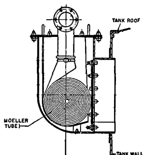
Fig. A-302 (b) (1). Cross-section Moeller Tube Chamber.
