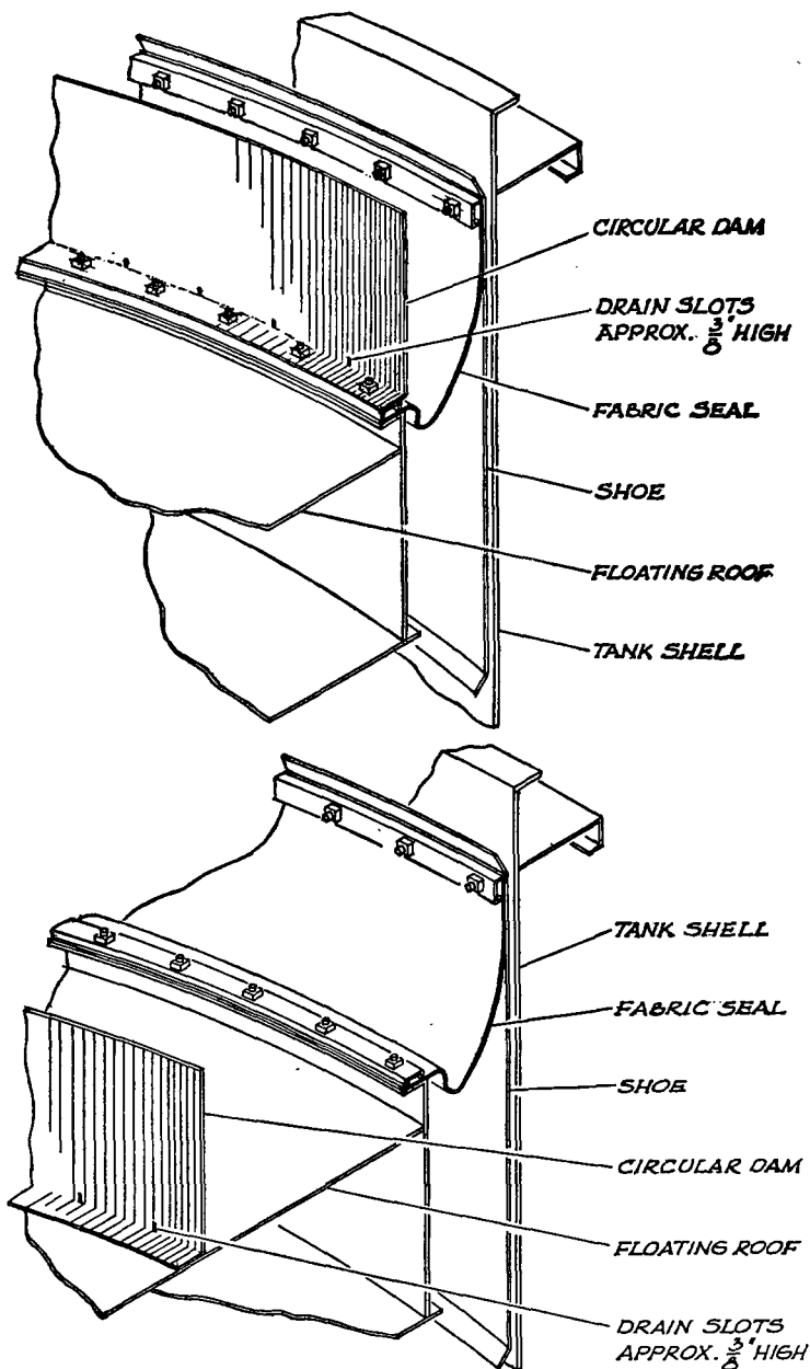
Fig. A-3311 (2). Typical Foam Dams for Floating Roof Tank Fixed Protection.
