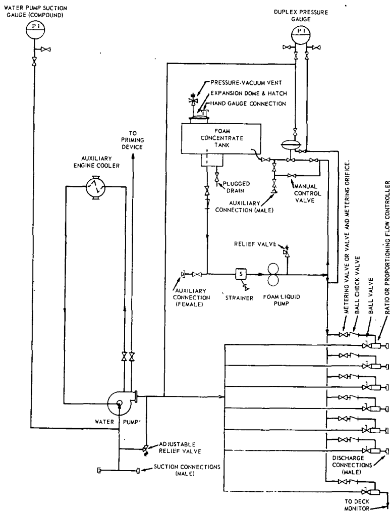
Fig. A-121(d). Balanced pressure proportioning.
