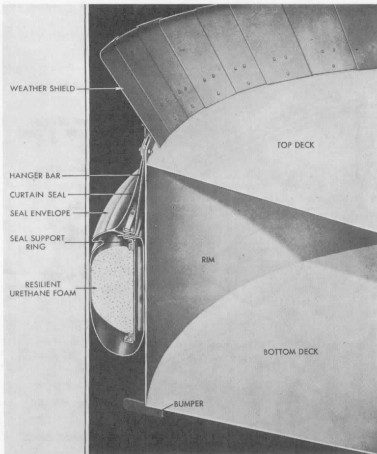
Fig. A-3311(2). Tube seal-open top floating roof tank.
