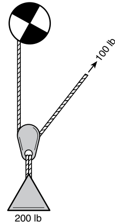
FIGURE A-1-4.175 Simple A 2:1 system.
