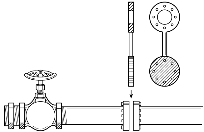
FIGURE A-7-1.2 Blanking or blinding.
