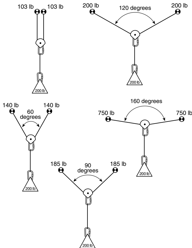
FIGURE A-1-4.44 The effect of angle forces on anchors and lines: critical angles.
