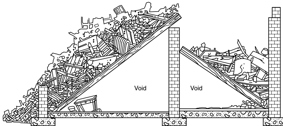
FIGURE A-1-4.27.2(e) A-frame floor collapse.
