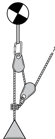
FIGURE A-1-4.4.2 Compound A 3:1 system (Z-Rig).
