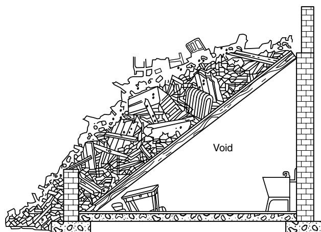
FIGURE A-1-4.27.2(a) Lean-to floor collapse. (Courtesy of U.S. Department of Civil Defense)
