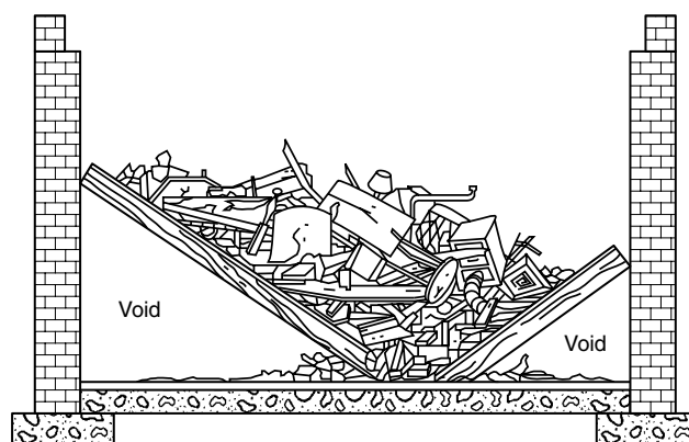
FIGURE A-1-4.27.2(b) V-shape floor collapse. (Courtesy of U.S. Department of Civil Defense)
