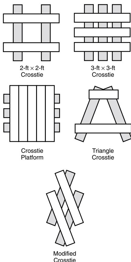
FIGURE A-8-1.15 Five basic configurations of cribbing.
