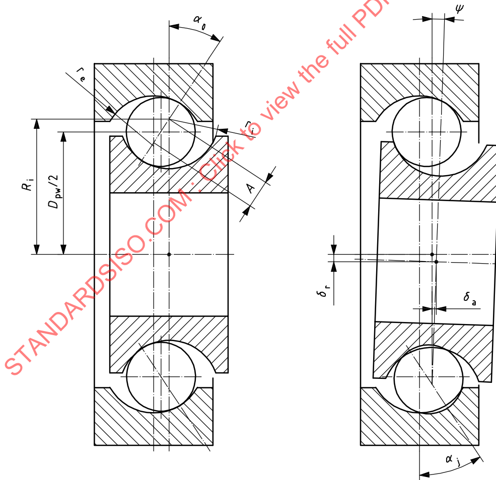
Figure 1 — Auxiliary geometry parameters
