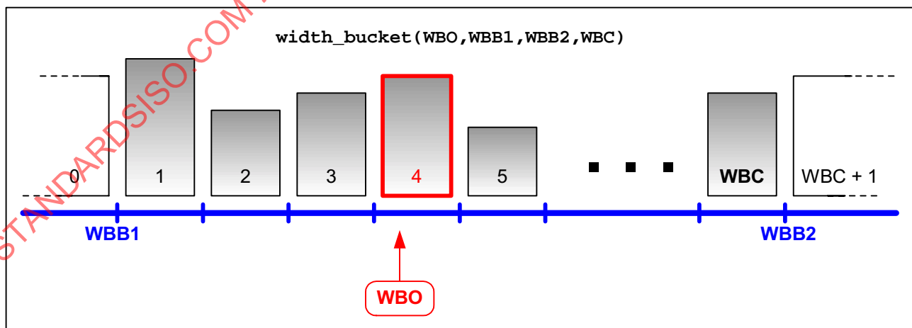
Figure 1— Illustration of WIDTH_BUCKET Semantics
