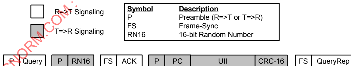
Figure Amd.1-24 — One tag reply
