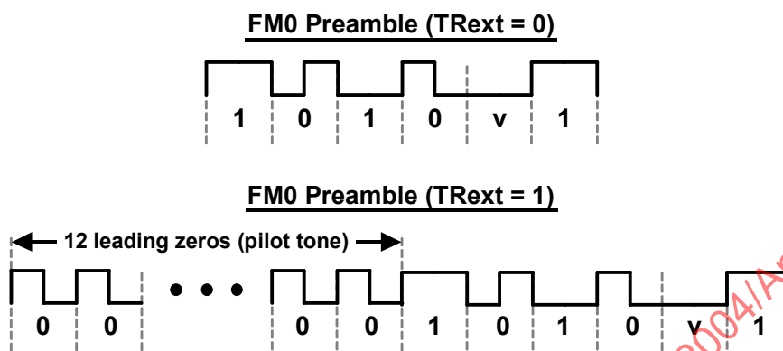
Figure Amd.1-14 — FM0 T=&gt;R preamble
