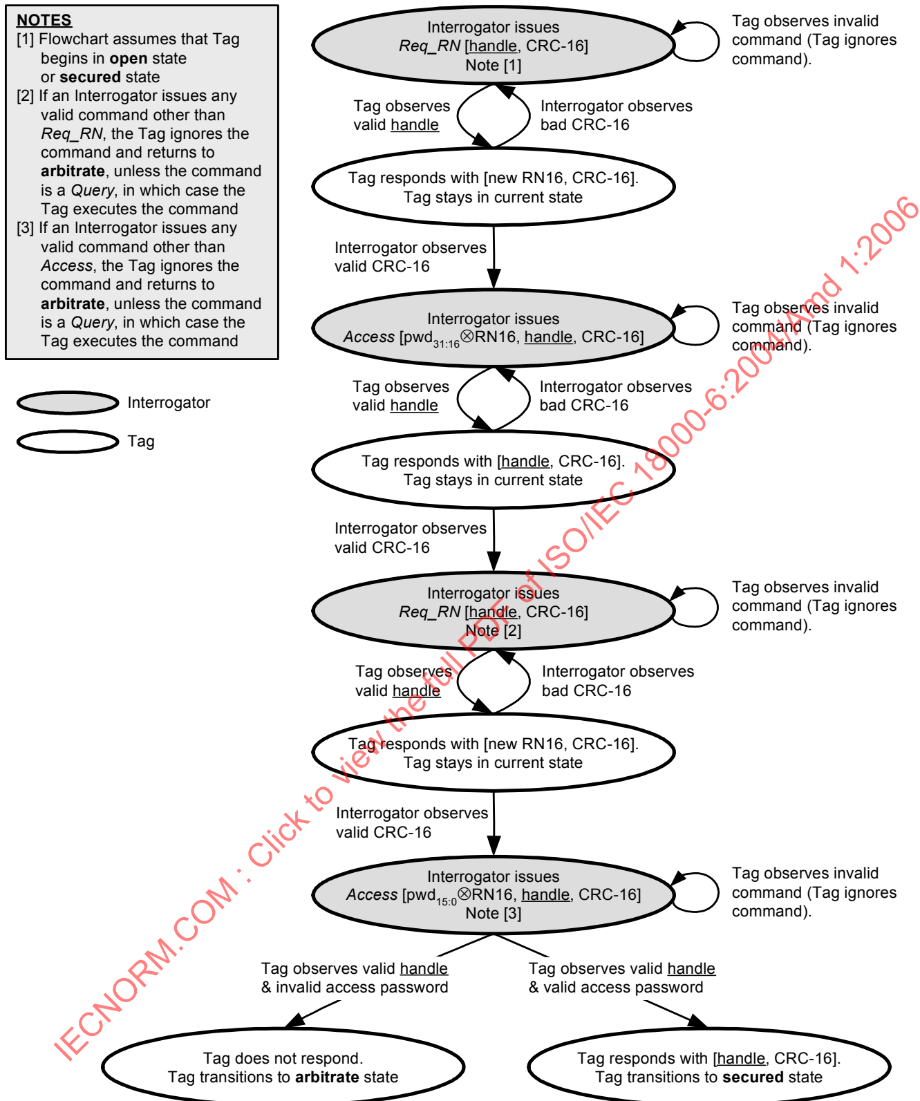
Figure Amd.1-28 — Access procedure
