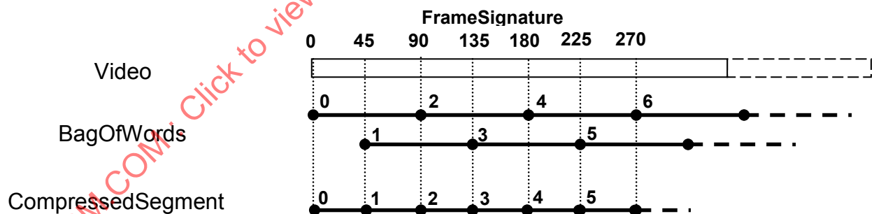
Figure Amd4-2 — Relationship between the BagOfWords and CompressedSegment temporal segments.
