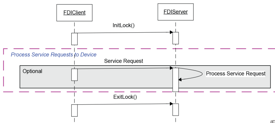
Figure 2 – Locking services
