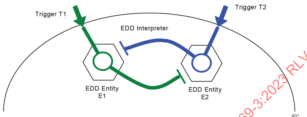
Figure C.6 – Concurrent execution of two triggers
