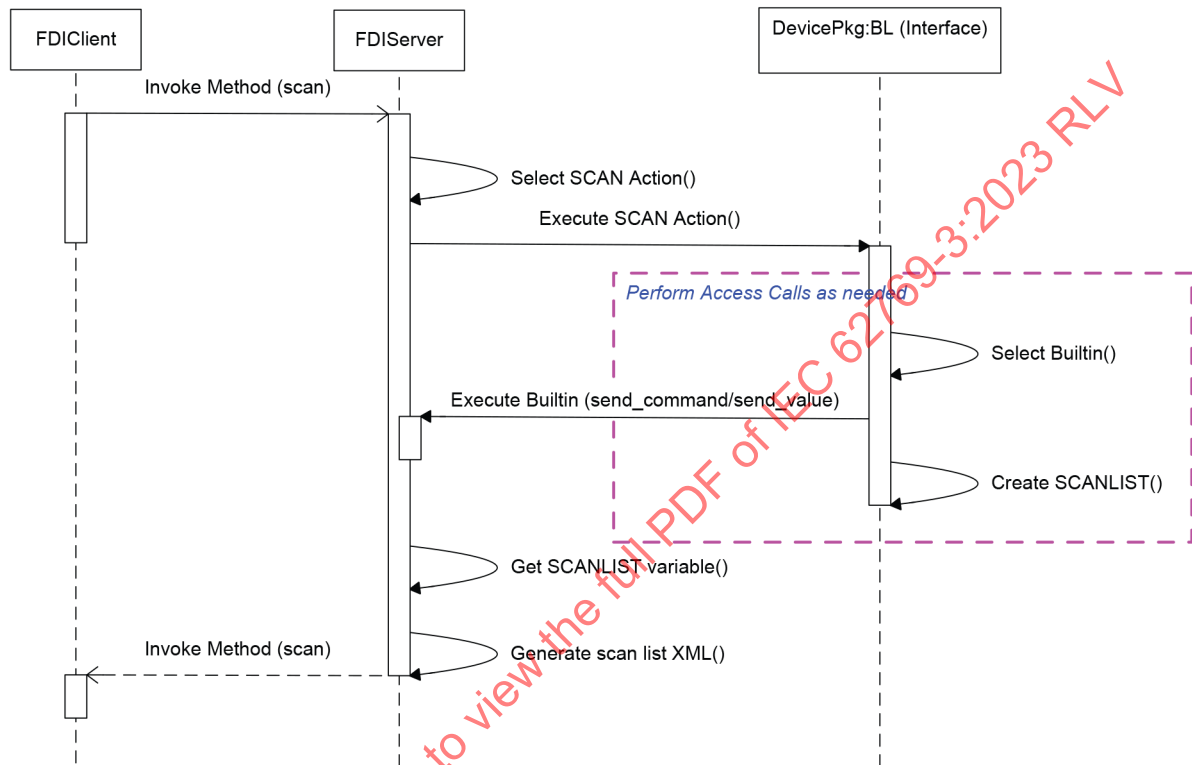
Figure 17 – Scan topology
