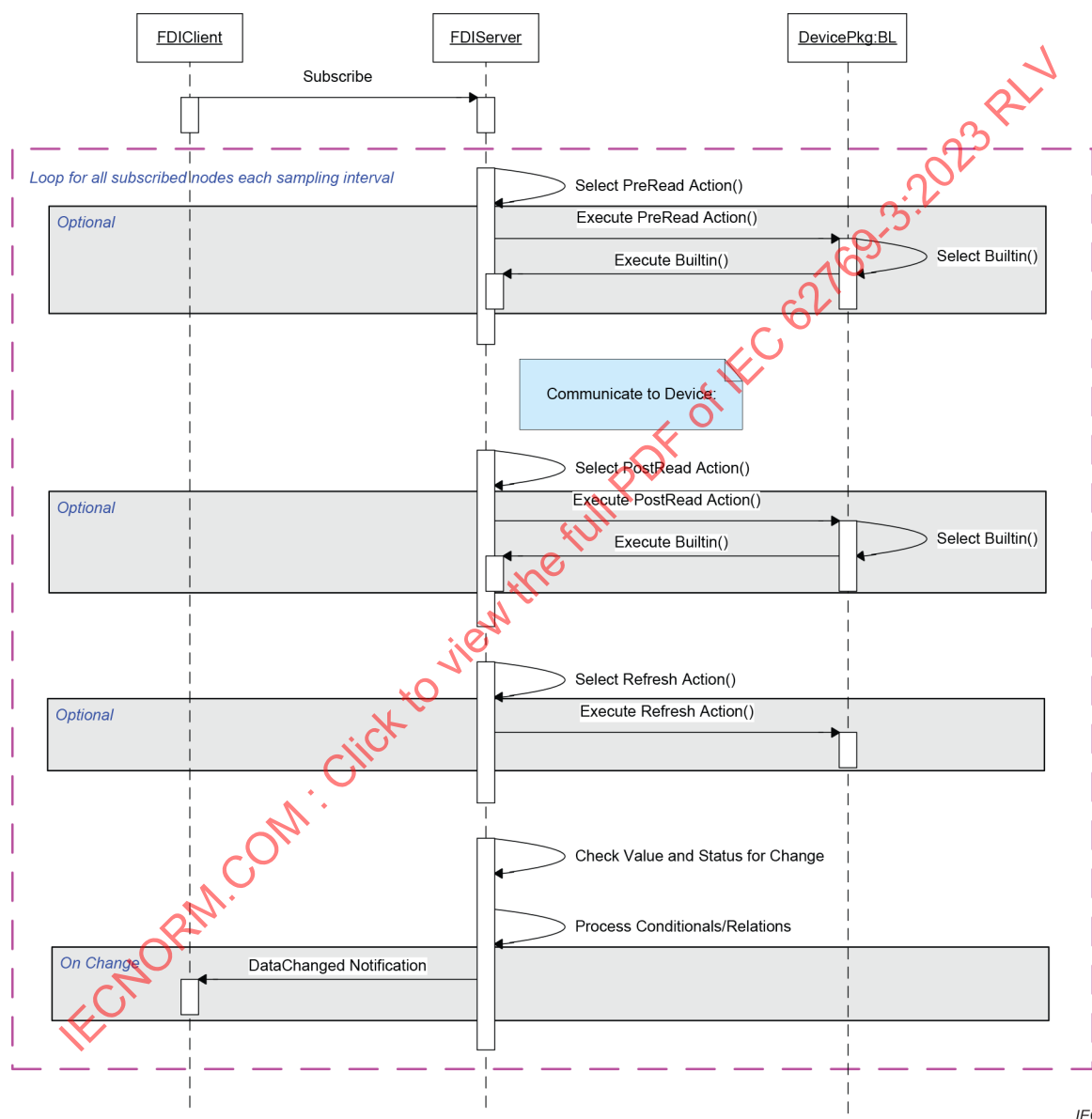
Figure 13 – Online variable subscription
