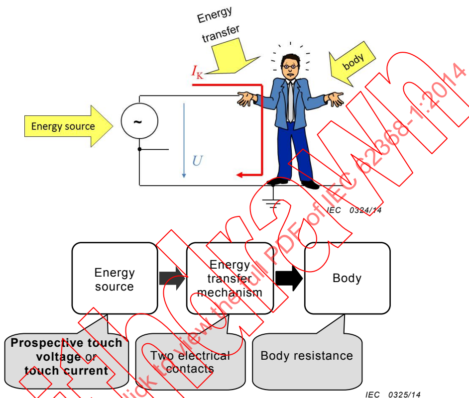
Figure 3 – Schematic and model for electrically-caused pain or injury
