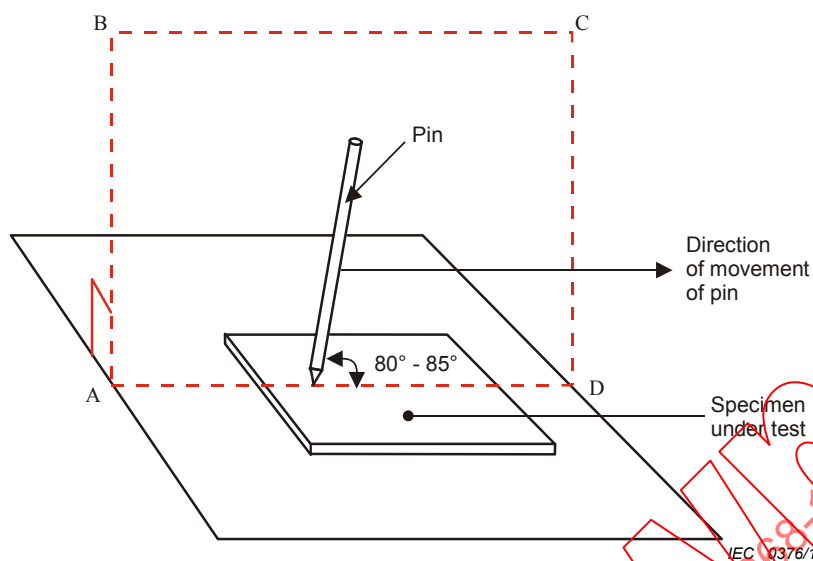
Figure G.3 – Abrasion resistance test for coating layers
