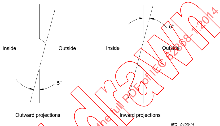
Figure P.2 – Examples of cross-sections of designs of side opening louvres which prevent vertical entry
