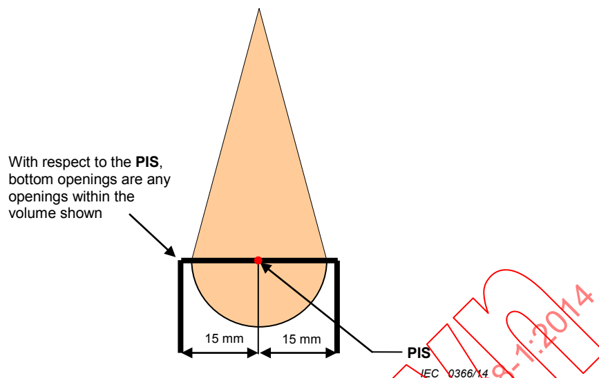
Figure 42 – Bottom openings
