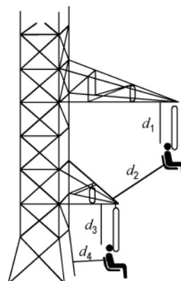
Figure 2 – Typical live working tasks
