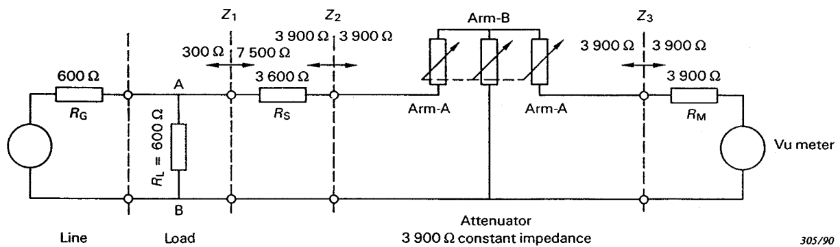
Figure 1 - Connection of the standard volume indicator
