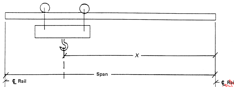
Fig. NUM-III-8344.1-1 Bridge Span (From CMAA 74)
