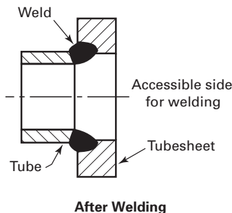
Figure 1 Full Penetration Weld
