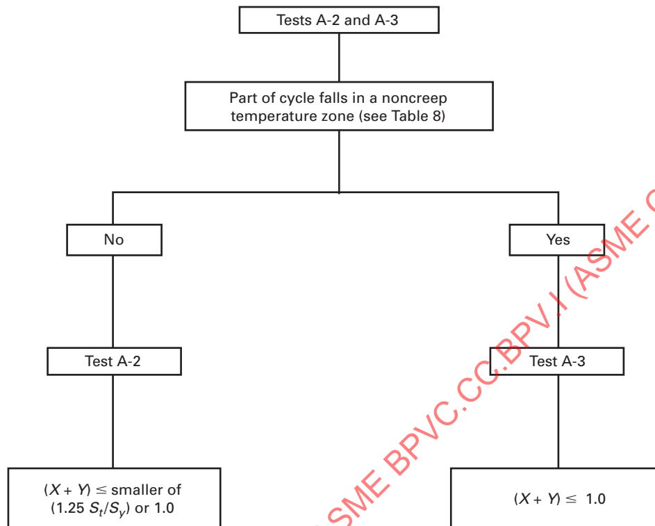
Figure 7 General Requirements for Tests A-2 and A-3
