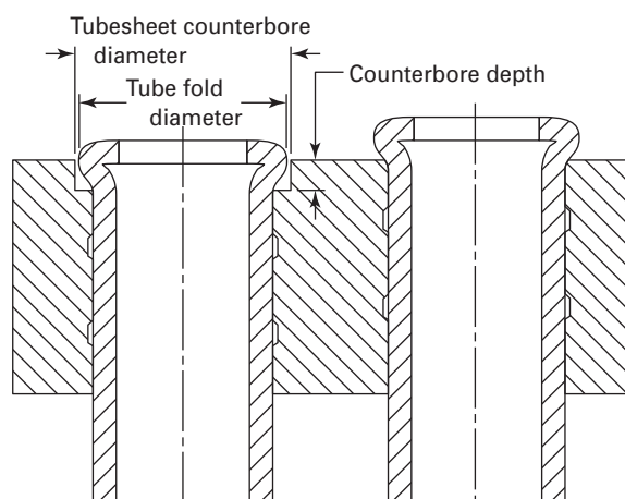
Figure 1 Typical Tube-to-Tubesheet Configurations Prior to Welding
