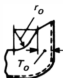
Figure F-2 Method of Establishing T_o When the Taper Encroaches on the Crotch Radius
