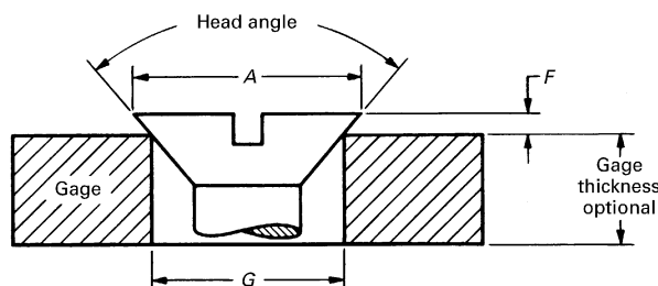
Fig. I-1 Protrusion Gage
