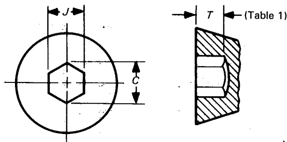
(a) Forged Hexagon Socket
