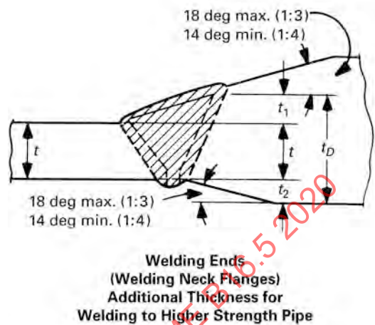
Figure 3 Bevel for Combined Thickness
