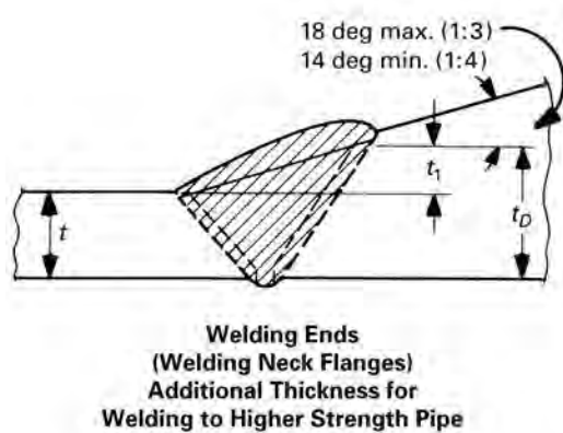
Figure 1 Bevel for Outside Thickness
