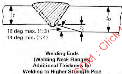
Figure 2 Bevel for Inside Thickness
