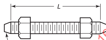
Stud Bolt With Nuts
