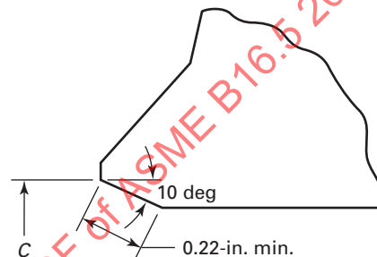
Fig. II-10 Inside Contour for Use With Taper Backing Ring
