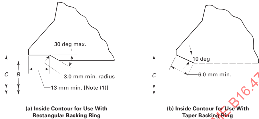
Fig. 2 Welding Ends (Welding Neck Flanges With Backing Rings)
